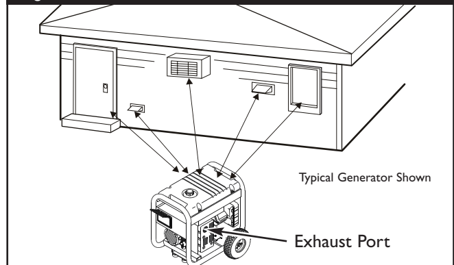
Figure 3 — Generator Clearance
